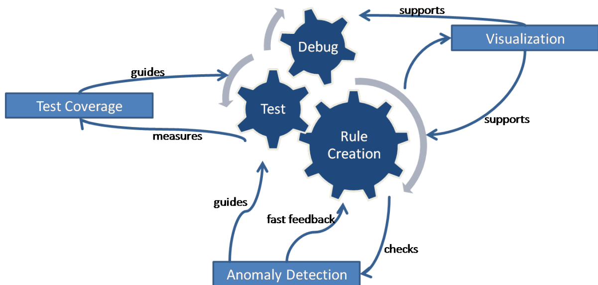
Figure 1: The overall architecture of tool support for the rule base development.
